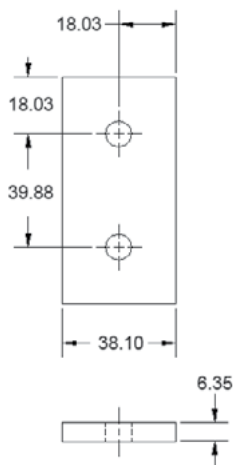
Joining Strips
