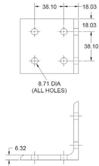
Corner Brackets
