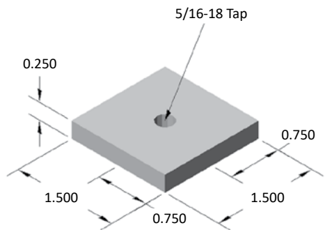
Component Dimensions:
